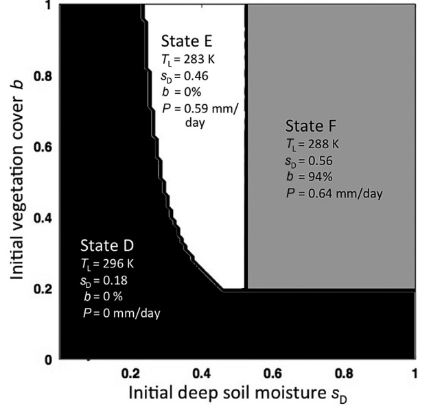
Fig. 3. Equilibrium potential temperature in the PBL for the parameter values indicated in the Appendix, as a function of the initial conditions on s_D (x-axis) and on b (y-axis). The black area indicates the equilibrium state \mathcal{D} (dry and hot, \theta_L \simeq 23^\circ\text{C} ), the white area indicates state \mathcal{E} (dry and cold, \theta_L \simeq 9.6^\circ\text{C} ), and the grey area indicate state \mathcal{F} (wet and temperate, \theta_L \simeq 15.3^\circ\text{C} ).
