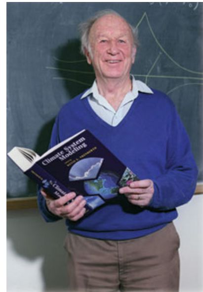
Ed Lorenz (1917 – 2008)
