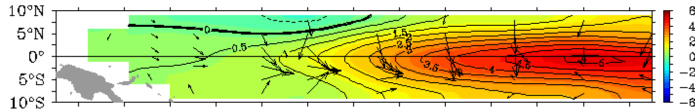
December 1997 Anomalies
