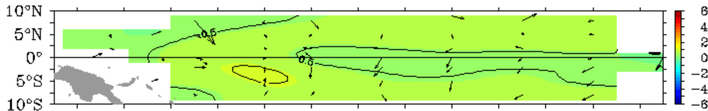
December 1993 Anomalies
