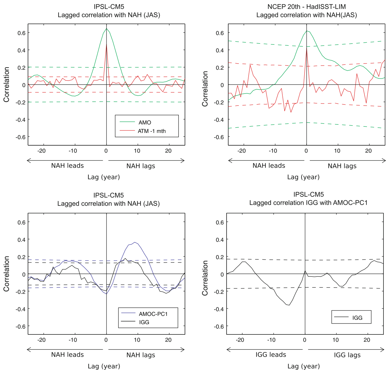
Fig. 13 Upper panel Temporal correlation between the NAH and the atmospheric forcing, and AMO in ( left panel ) IPSL-CM5 and ( right panel ) twentieth century NCEP reanalysis and HadISST-LIM. Lower-left panel Temporal correlation between the NAH and the PC1 of the yearly AMOC (AMOC-PC1) and the intergyre gyre index (IGG) in IPSL-CM5. Lower-right panel Temporal correlation between the
