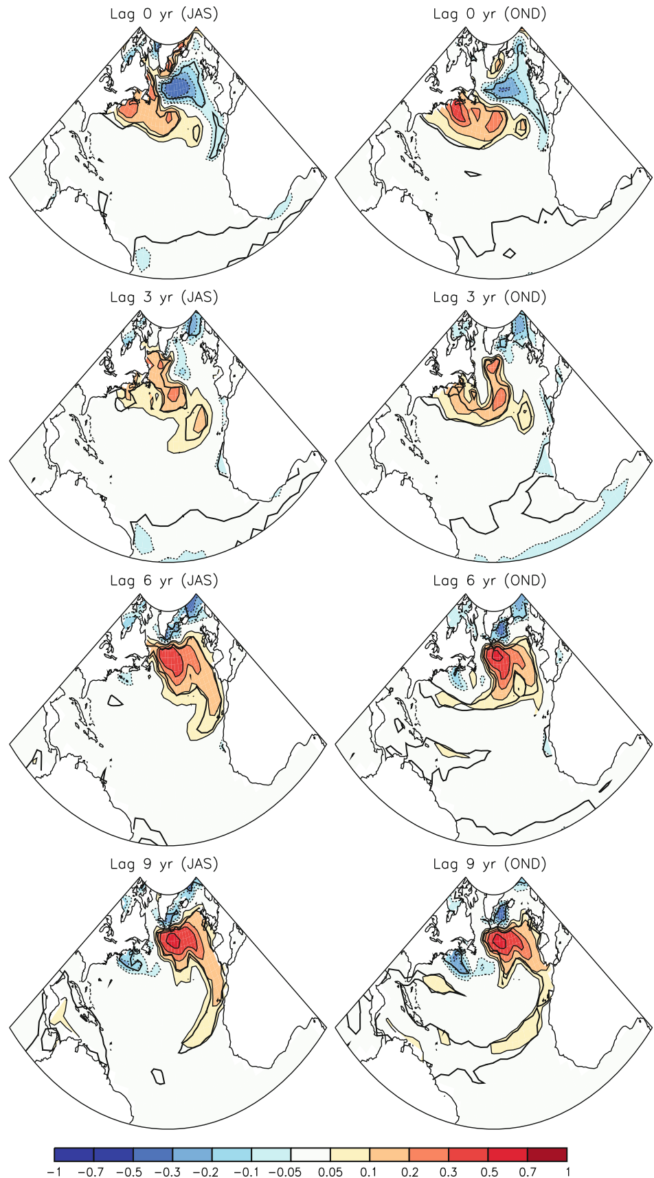
Fig. 6 SST (in K) regression onto normalized AMOC-PC1 in IPSL-CM5, for ( left panel ) summer (JAS) and ( right panel ) fall (OND). The lag (in year) is positive when AMOC-PC1 leads. The thick black lines indicate the 5 % significance, given by Monte Carlo analysis
