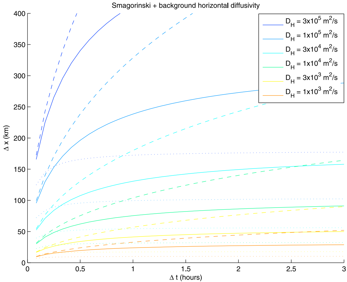
Figure 5. Relationship between time and space resolutions corresponding to different values of horizontal diffusivity estimated using a mesoscale (MM5) model setup and shears of 0.1, 1, and 10 \text{day}^{-1} (dashed, solid, and pointed lines, respectively). MOCAGE parameters yield a horizontal diffusivity above 10^5 \text{ m}^2 \text{ s}^{-1} . See text for details.
