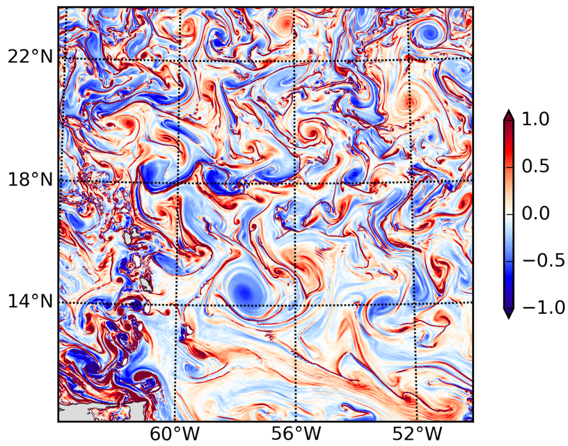
A Sea Surface Relative Vorticity snapshot from the MegaAtl simulation by Jonathan Gula
