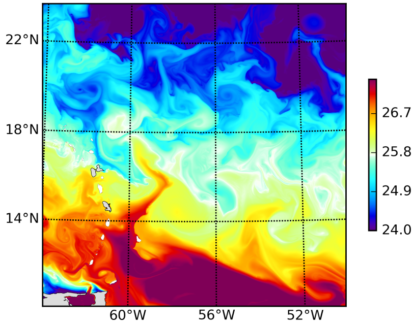
A Sea Surface Temperature snapshot from the MegaAtl simulation by Jonathan Gula
