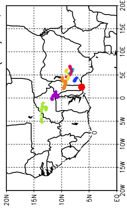
Ballons laches a J+60 h (10/05, 12 UTC)
