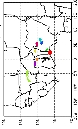
Ballons laches a J+42 h (09/05, 18 UTC)
