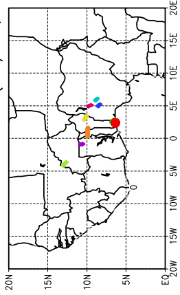
Ballons laches a J+48 h (10/05, 00 UTC)
