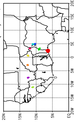
Ballons laches a J+24 h (09/05, 00 UTC)
