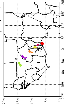
Ballons laches a J+90 h (18/05, 18 UTC)
