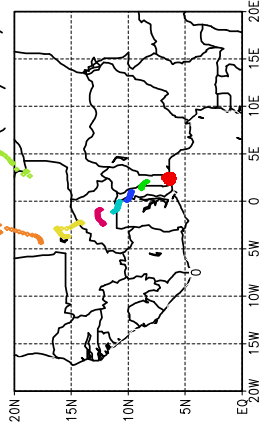
Ballons laches a J+24 h (16/05, 00 UTC)
