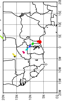
Ballons laches a J+18 h (15/05, 18 UTC)
