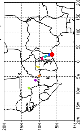
Ballons laches a J+66 h (17/05, 18 UTC)
