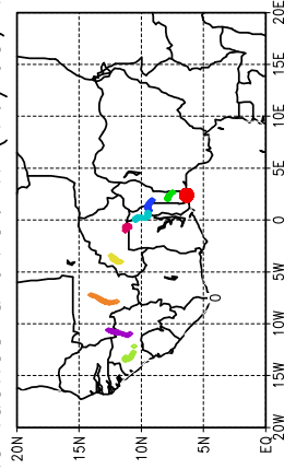
Ballons laches a J+36 h (16/05, 12 UTC)
