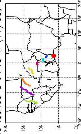
Ballons laches a J+48 h (17/05, 00 UTC)
