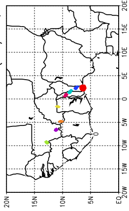
Ballons laches a J+60 h (17/05, 12 UTC)
