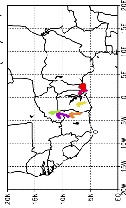
Ballons laches a J+84 h (22/05, 00 UTC)
