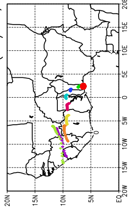
Ballons laches a J+42 h (20/05, 6 UTC)
