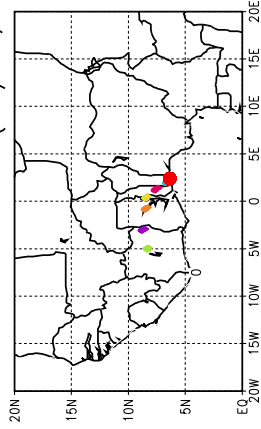
Ballons laches a J+84 h (28/05, 00 UTC)
