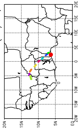
Ballons laches a J+36 h (26/05, 12 UTC)
