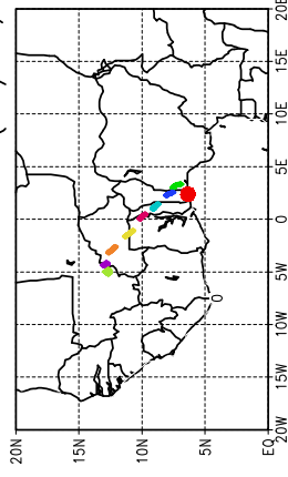
Ballons laches a J+30 h (26/05, 6 UTC)
