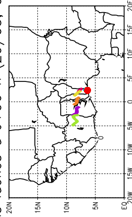
Ballons laches a J+96 h (29/05, 00 UTC)
