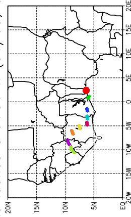
Ballons laches a J+36 h (31/05, 00 UTC)
