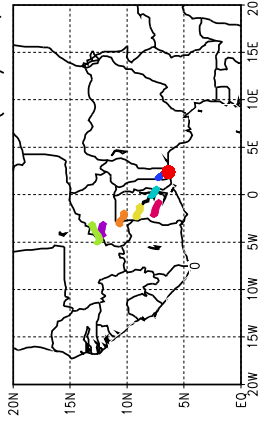
Ballons laches a J+66 h (01/06, 6 UTC)
