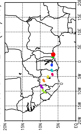
Ballons laches a J+42 h (31/05, 6 UTC)
