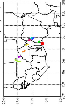
Ballons laches a J+42 h (04/06, 18 UTC)
