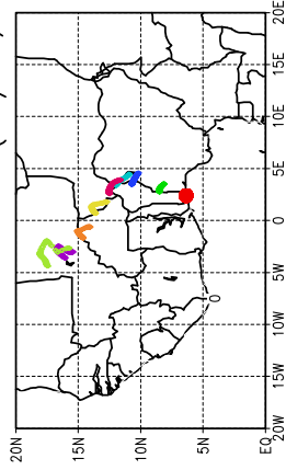
Ballons laches a J+36 h (04/06, 12 UTC)
