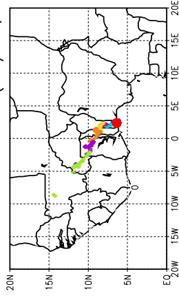
Ballons laches a J+72 h (08/06, 00 UTC)
