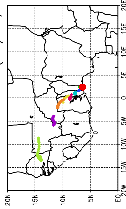
Ballons laches a J+36 h (06/06, 12 UTC)
