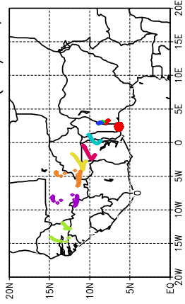
Ballons laches a J+12 h (05/06, 12 UTC)
