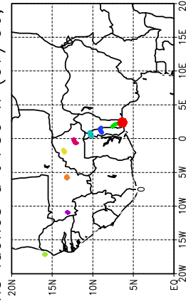
Ballons laches a J+30 h (07/06, 6 UTC)
