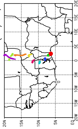
Ballons laches a J+36 h (14/06, 12 UTC)
