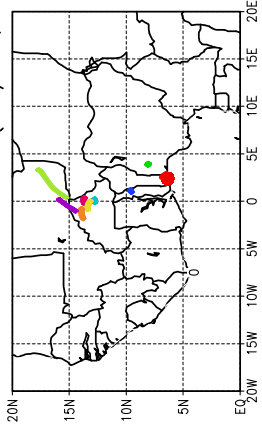
Ballons laches a J+24 h (18/06, 00 UTC)
