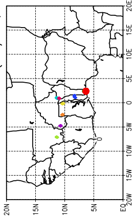
Ballons laches a J+48 h (19/06, 00 UTC)
