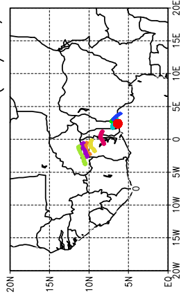
Ballons laches a J+36 h (20/06, 12 UTC)
