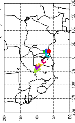
Ballons laches a J+24 h (20/06, 00 UTC)
