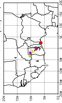
Ballons laches a J+84 h (22/06, 12 UTC)
