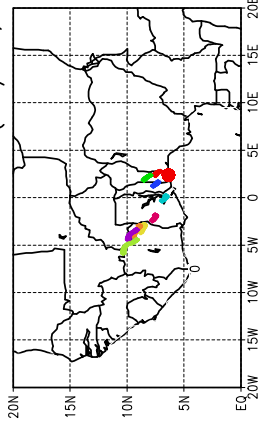
Ballons laches a J+18 h (19/06, 18 UTC)
