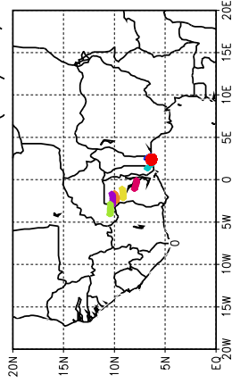
Ballons laches a J+72 h (22/06, 00 UTC)
