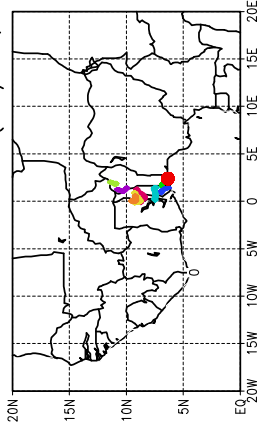
Ballons laches a J+36 h (24/06, 00 UTC)
