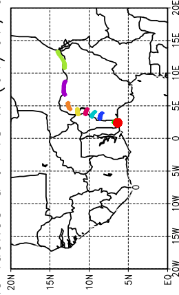
Ballons laches a J+48 h (01/07, 00 UTC)
