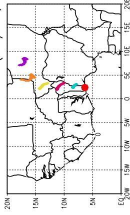
Ballons laches a J+78 h (16/05, 6 UTC)
