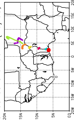
Ballons laches a J+90 h (16/05, 18 UTC)
