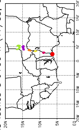
Ballons laches a J+96 h (17/05, 00 UTC)
