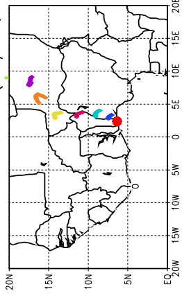
Ballons laches a J+66 h (15/05, 18 UTC)
