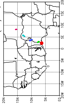
Ballons laches a J+42 h (15/05, 18 UTC)
