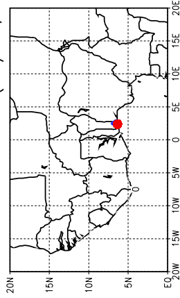
Ballons laches a J+72 h (18/05, 12 UTC)
