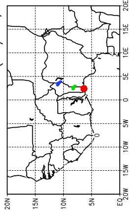
Ballons laches a J+36 h (17/05, 00 UTC)
