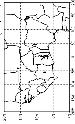
Ballons laches a J+90 h (19/05, 6 UTC)
