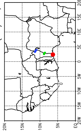
Ballons laches a J+30 h (16/05, 18 UTC)
