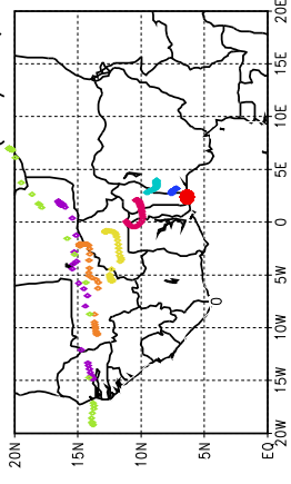
Ballons laches a J+66 h (18/05, 18 UTC)
