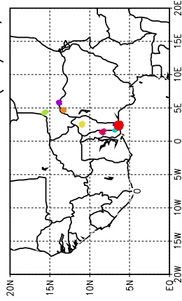
Ballons laches a J+72 h (23/05, 00 UTC)
