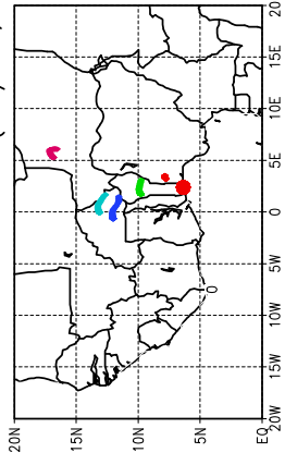
Ballons laches a J+18 h (20/05, 18 UTC)
