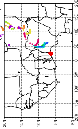
Ballons laches a J+24 h (21/05, 00 UTC)
