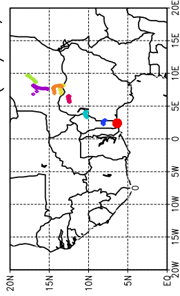
Ballons laches a J+36 h (23/05, 00 UTC)
