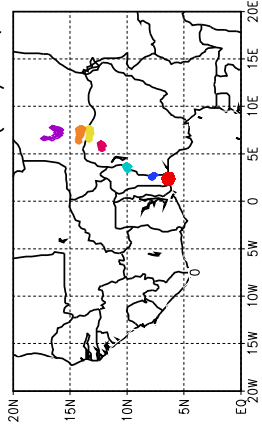
Ballons laches a J+60 h (24/05, 00 UTC)
