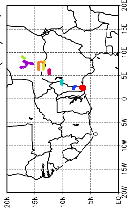
Ballons laches a J+24 h (22/05, 12 UTC)
