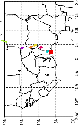
Ballons laches a J+90 h (25/05, 6 UTC)
