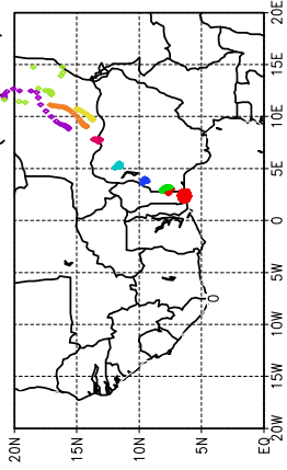
Ballons laches a J+12 h (22/05, 00 UTC)
