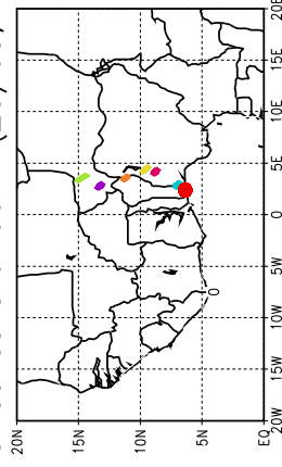
Ballons laches a J+90 h (25/05, 18 UTC)
