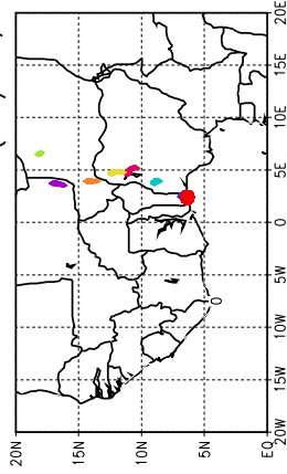
Ballons laches a J+72 h (25/05, 00 UTC)
