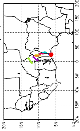
Ballons laches a J+72 h (29/05, 00 UTC)
