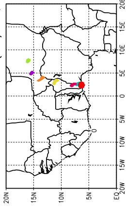
Ballons laches a J+90 h (02/06, 6 UTC)
