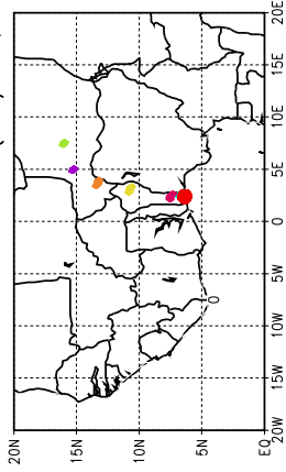
Ballons laches a J+96 h (02/06, 12 UTC)
