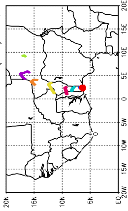
Ballons laches a J+72 h (01/06, 12 UTC)
