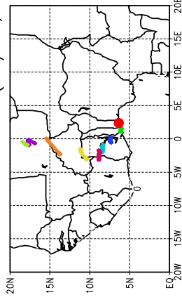
Ballons laches a J+30 h (30/05, 18 UTC)
