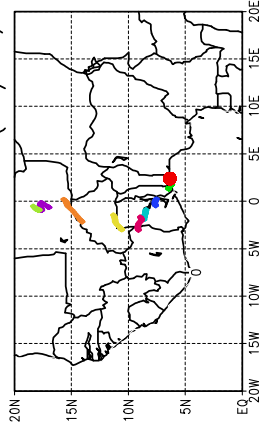
Ballons laches a J+36 h (31/05, 00 UTC)
