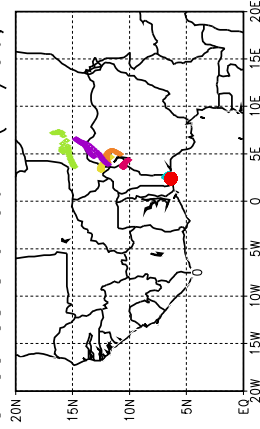
Ballons laches a J+96 h (11/06, 12 UTC)
