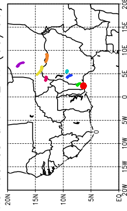
Ballons laches a J+42 h (09/06, 6 UTC)
