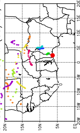
Ballons laches a J+36 h (09/06, 00 UTC)
