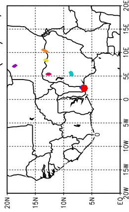
Ballons laches a J+72 h (10/06, 12 UTC)
