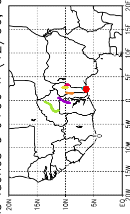
Ballons laches a J+96 h (12/06, 00 UTC)
