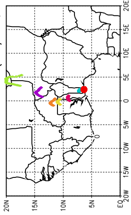
Ballons laches a J+84 h (22/06, 12 UTC)
