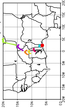
Ballons laches a J+72 h (22/06, 00 UTC)
