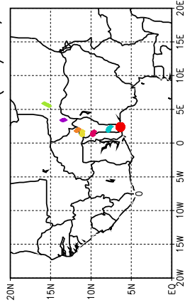
Ballons laches a J+84 h (23/06, 00 UTC)
