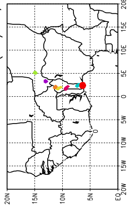
Ballons laches a J+90 h (23/06, 6 UTC)
