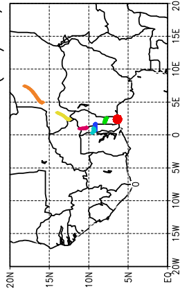
Ballons laches a J+30 h (22/06, 6 UTC)
