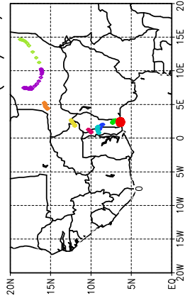
Ballons laches a J+42 h (22/06, 18 UTC)
