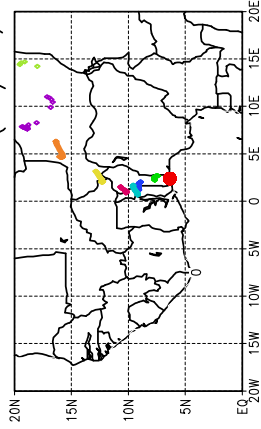
Ballons laches a J+36 h (22/06, 12 UTC)
