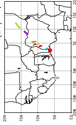
Ballons laches a J+90 h (26/06, 18 UTC)
