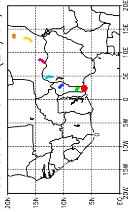
Ballons laches a J+36 h (26/06, 00 UTC)
