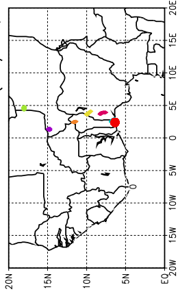
Ballons laches a J+96 h (14/05, 00 UTC)
