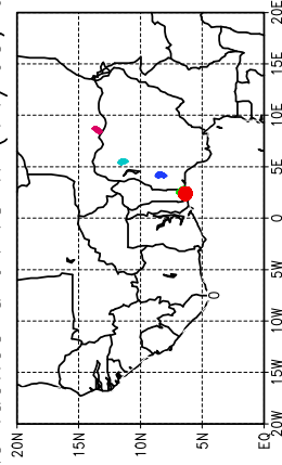
Ballons laches a J+48 h (14/05, 00 UTC)
