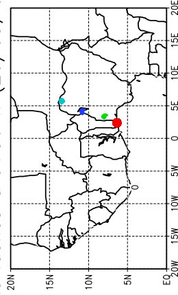
Ballons laches a J+36 h (20/05, 00 UTC)
