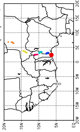
Ballons laches a J+60 h (21/05, 00 UTC)
