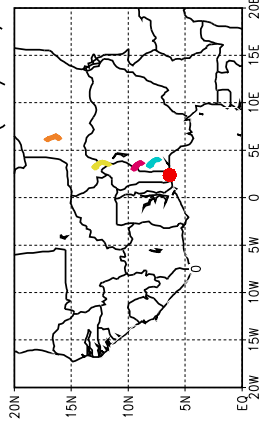
Ballons laches a J+78 h (21/05, 18 UTC)
