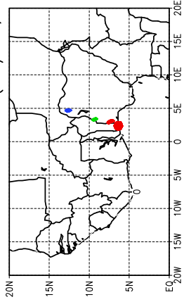
Ballons laches a J+12 h (19/05, 00 UTC)
