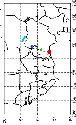
Ballons laches a J+24 h (19/05, 12 UTC)
