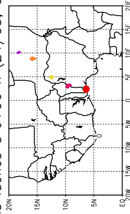
Ballons laches a J+96 h (24/05, 00 UTC)
