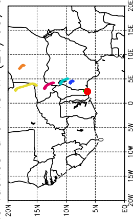
Ballons laches a J+48 h (26/05, 00 UTC)
