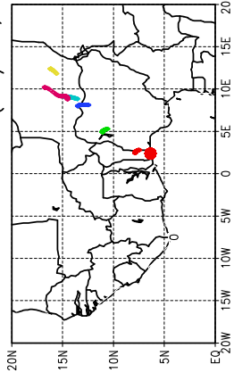
Ballons laches a J+18 h (24/05, 18 UTC)
