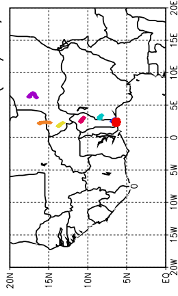
Ballons laches a J+72 h (27/05, 00 UTC)
