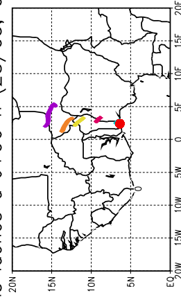
Ballons laches a J+96 h (28/05, 00 UTC)
