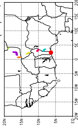
Ballons laches a J+78 h (06/06, 6 UTC)
