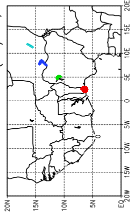
Ballons laches a J+24 h (04/06, 00 UTC)
