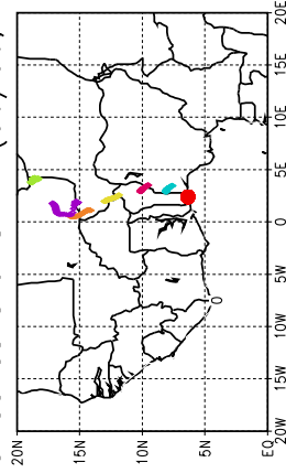
Ballons laches a J+84 h (06/06, 12 UTC)
