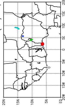
Ballons laches a J+30 h (04/06, 6 UTC)
