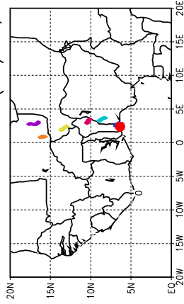
Ballons laches a J+72 h (06/06, 00 UTC)
