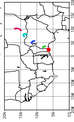
Ballons laches a J+42 h (04/06, 18 UTC)
