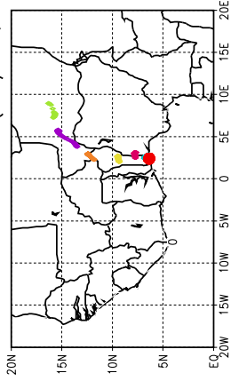
Ballons laches a J+96 h (14/06, 00 UTC)
