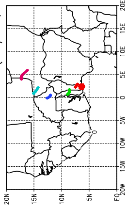
Ballons laches a J+12 h (10/06, 12 UTC)
