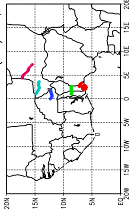
Ballons laches a J+18 h (10/06, 18 UTC)
