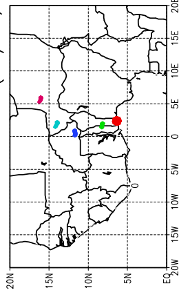
Ballons laches a J+30 h (11/06, 6 UTC)
