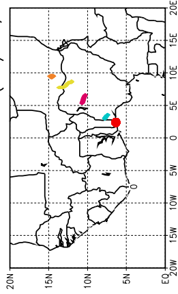
Ballons laches a J+84 h (16/06, 00 UTC)
