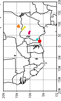
Ballons laches a J+90 h (16/06, 6 UTC)
