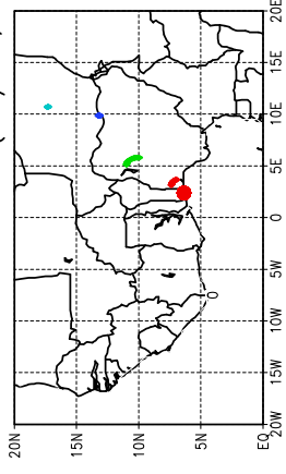
Ballons laches a J+18 h (15/06, 18 UTC)
