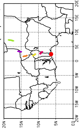
Ballons laches a J+96 h (19/06, 00 UTC)
