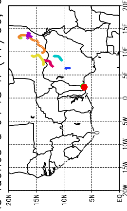
Ballons laches a J+48 h (17/06, 00 UTC)
