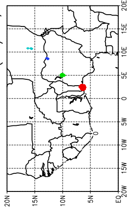
Ballons laches a J+24 h (16/06, 00 UTC)
