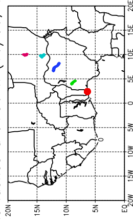
Ballons laches a J+36 h (16/06, 12 UTC)
