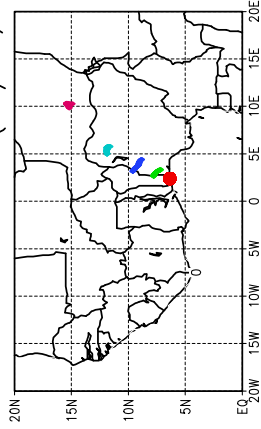
Ballons laches a J+36 h (23/06, 12 UTC)
