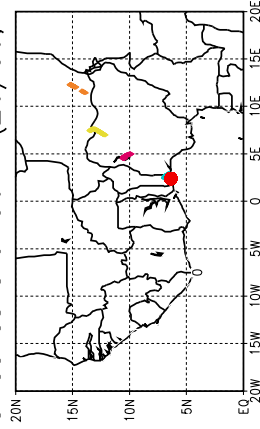
Ballons laches a J+96 h (26/06, 12 UTC)
