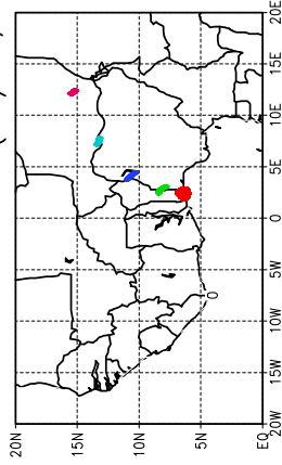
Ballons laches a J+24 h (23/06, 12 UTC)
