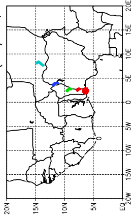
Ballons laches a J+12 h (23/06, 00 UTC)
