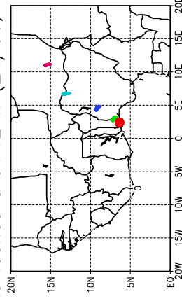
Ballons laches a J+42 h (24/06, 18 UTC)
