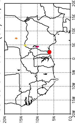
Ballons laches a J+96 h (30/06, 00 UTC)
