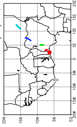
Ballons laches a J+12 h (28/06, 00 UTC)
