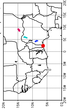
Ballons laches a J+60 h (30/06, 00 UTC)
