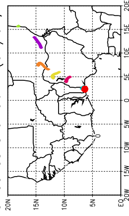
Ballons laches a J+96 h (01/07, 12 UTC)
