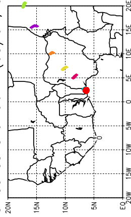
Ballons laches a J+96 h (03/07, 00 UTC)
